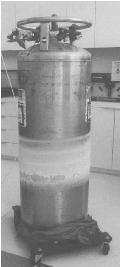
Figure 4.6 Ice will form on the liquid nitrogen container if high nitrogen flow rates are maintained over long periods.
