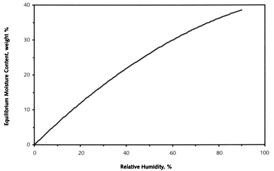
Figure 3.5 Sorption isotherm of bead-type silica gel
