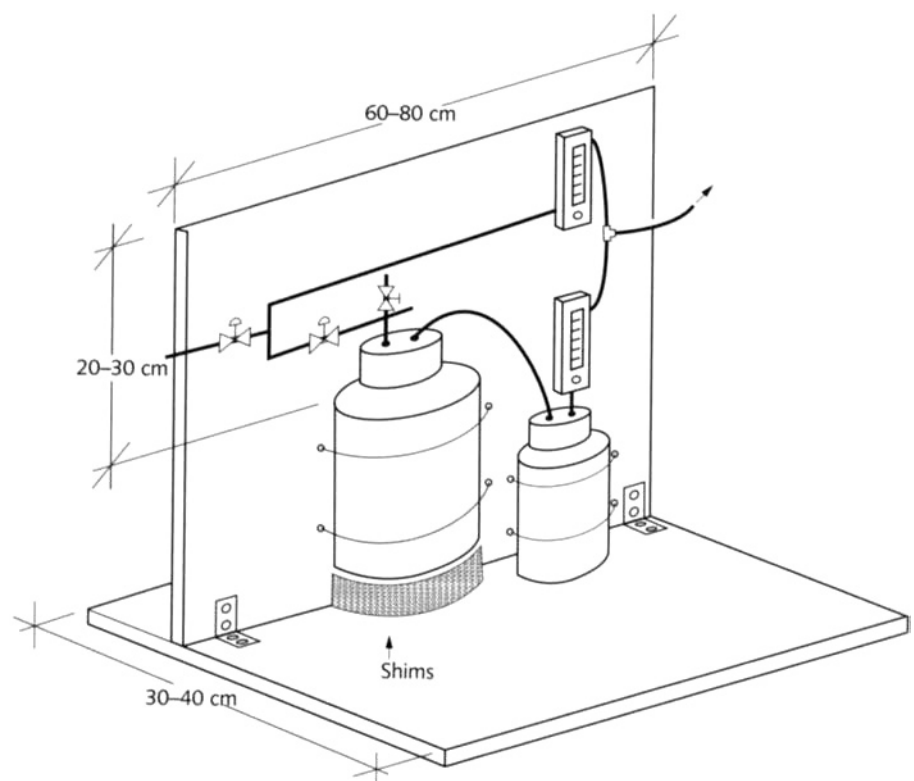
Figure I.4 Schematic of a plywood mounting of the humidification unit
